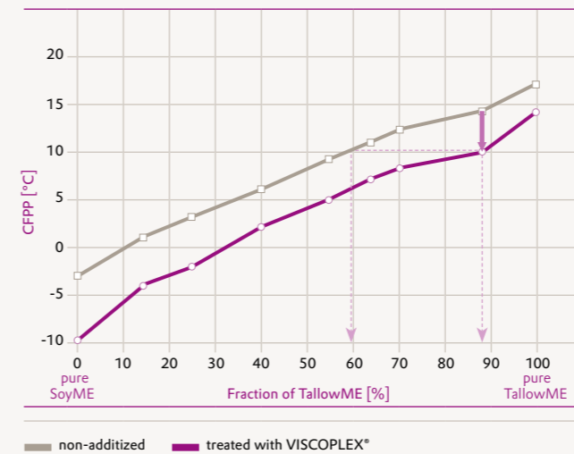
Cost Saving with VISCOPLEX® in TME-SME Blends (Txx)
